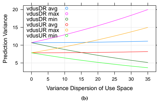
Figure 3: Comparison of D-optimal and U-optimal designs with right censoring using (a) FUS plot and (b) VDUS plot.
