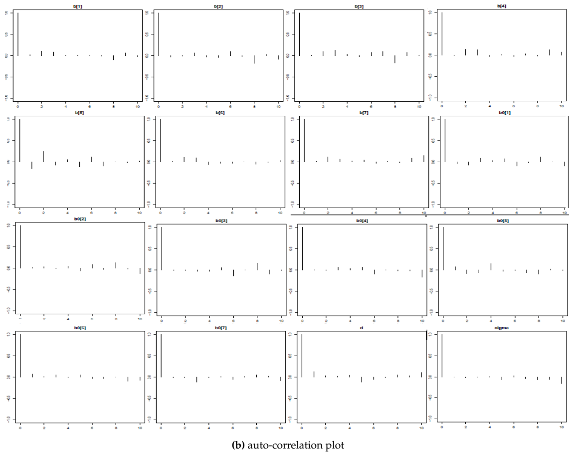
Figure A5: Trace and auto-correlation plots in the zoib-fixed model in Example 1.
